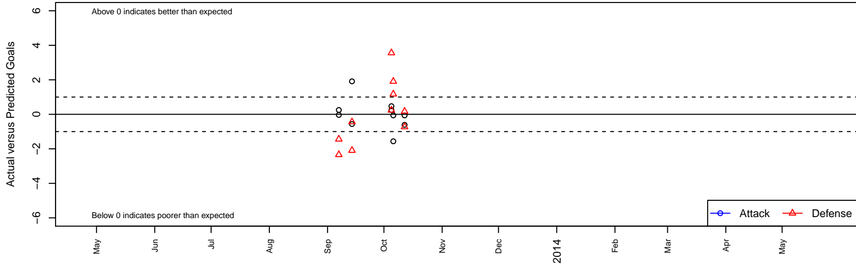
PVSC United Blitz G00 Dots are actual minus expected GF (blue circles) and GA (red triangles). Blue line is smoothed change in attack strength. Red is smoothed change in defense strength.
